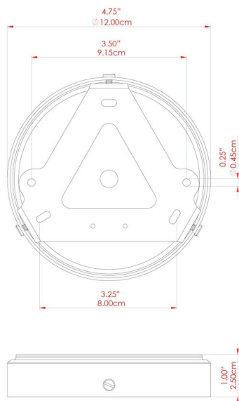
FIXING BRACKET: MLROSE39 | Racing Green
