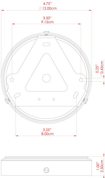
FIXING BRACKET: MLWB17 | PC Mint Turquoise
