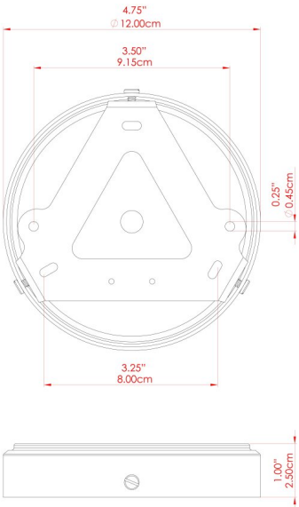
FIXING BRACKET: MLWB17 | PC Mustard Honey Yellow
