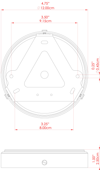
FIXING BRACKET: MLWB17
