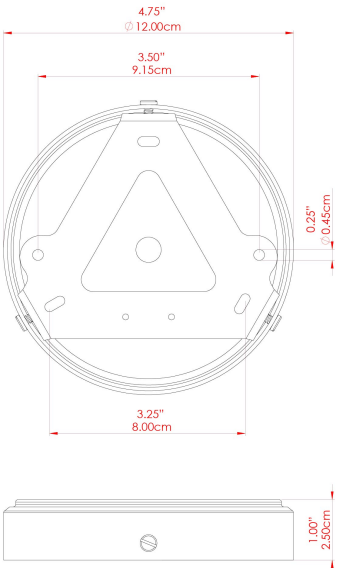
FIXING BRACKET: MLROSE39 | Matt Honey Yellow
