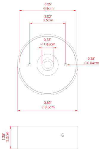
FIXING BRACKET: MLWB13 | Natural Brass
