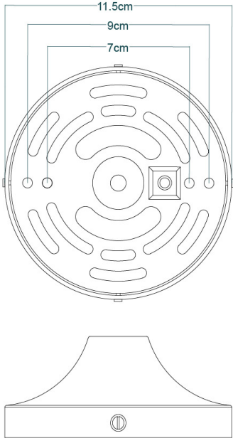
Fixing Bracket MLWB12 * Fixing bracket may differ for UL wired products.
