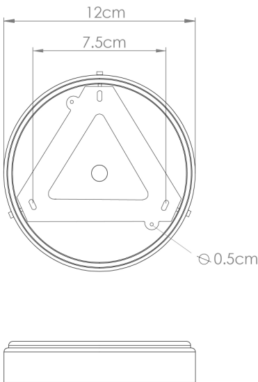
Fixing Bracket MLWB17| Antique Brass
