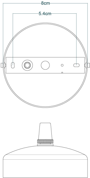
FIXING BRACKET: MLROSE10 | Polished Chrome
