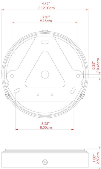
FIXING BRACKET: MLROSE39
