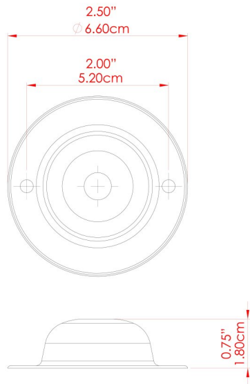
FIXING BRACKET: MLWB04 | Matt Vanilla Cream
