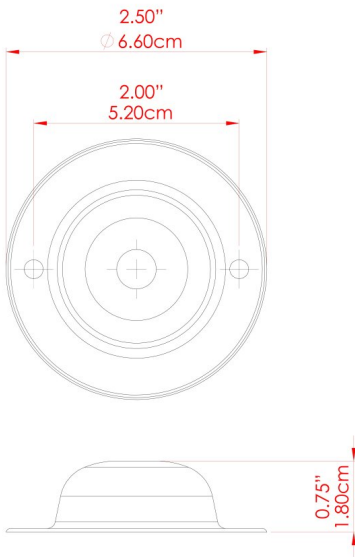
FIXING BRACKET: MLWB04 | Antique Brass
