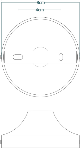
Fixing Bracket MLWB03 | White * Fixing bracket may differ for UL wired products.
