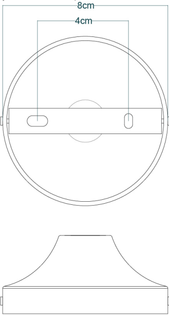
Fixing Bracket MLWB03 | Matt Black * Fixing bracket may differ for UL wired products.
