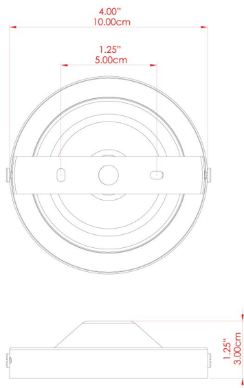
FIXING BRACKET: MLWB02 | Satin Brass
