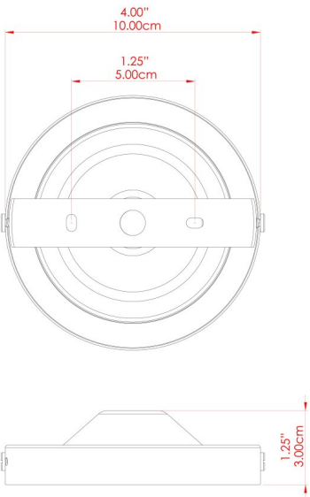
FIXING BRACKET: MLWB02 | Antique Brass
