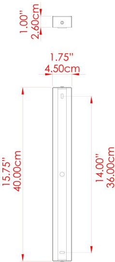
FIXING BRACKET: MLWB07 | Orange
